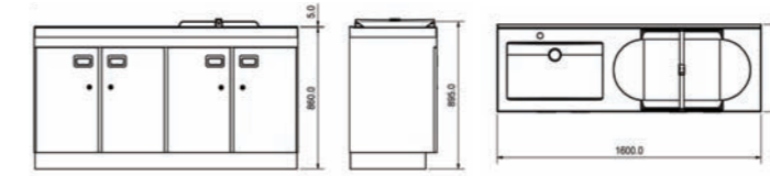
BC1604D L/R Baby Changing station with 4 lockable doors and removable storage panel
