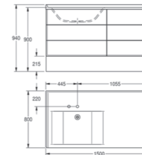
AQRM 700 Baby Changing station with drawers
